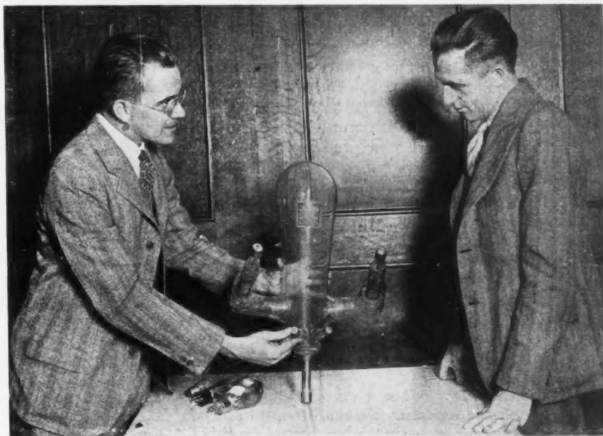
The family of mercury-vapor three-element electronic tubes variously known as "grid-glow" tubes, "thyatrons," etc., will find many new important industrial applications during 1931. The tube shown breaks a welding current of 75 kw. 500 times per minute
