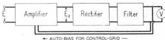
Fig. 2—Using the 551E exponential tube for logarithmic indication
