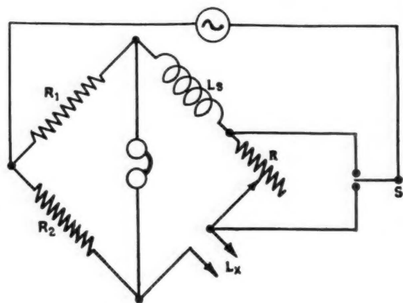
Fig. 1—The familiar Wheatstone bridge circuit
