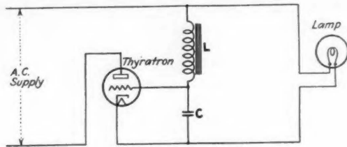
Fig. 4—Electron tube flasher circuit
