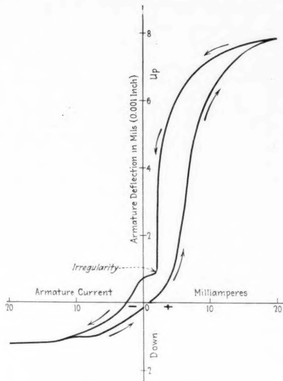
Fig. 1—Irregularity in speaker response
