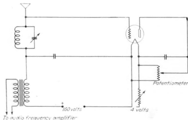
Receiver for ultra-short waves; note positive grid
