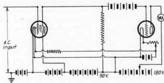
Fig. 2—An amplifier-detector for bridge work
