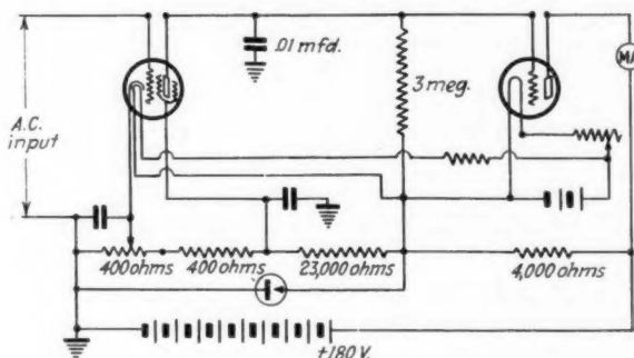
Fig. 3—Addition of voltage regulator and self-bias apparatus
