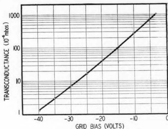
Fig. 1—Relation between transconductance and control grid bias in an exponential tetrode
