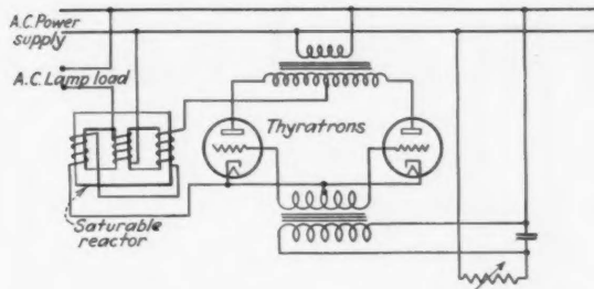
Fig. 8—Illumination control by electron tubes
