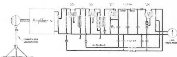
Fig. 4—Diagram of logarithmic indicator for use in automatic recording of sound-pressure frequency characteristics of loud-speakers
