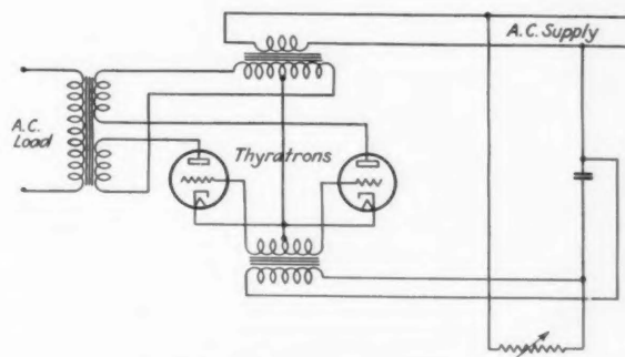
Fig. 7—Variable a.c. output secured by resistance control
