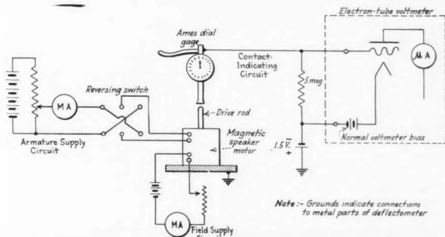
Fig. 4—Details of circuit for measuring deflections
