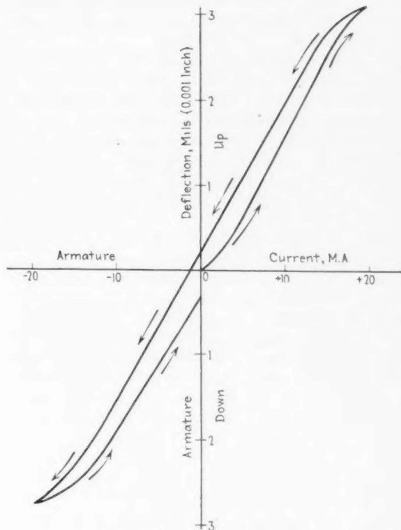
Fig. 2—Evidence of improved speaker characteristic; narrow, regular loops
