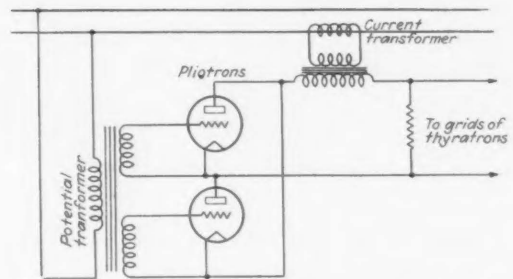
Fig. 1—Pliotron phase-controlled circuit
