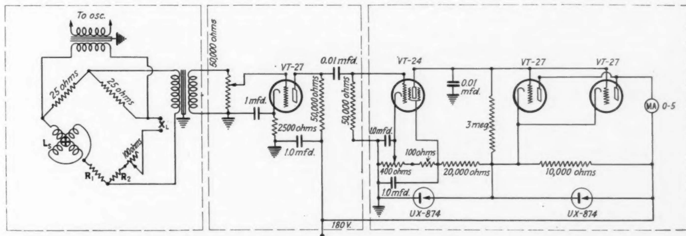
Fig. 4—The complete circuit diagram of the instrument. The power supply may be a conventional rectifier-filter system
