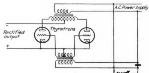
Fig. 6—Variable output secured by resistance control
