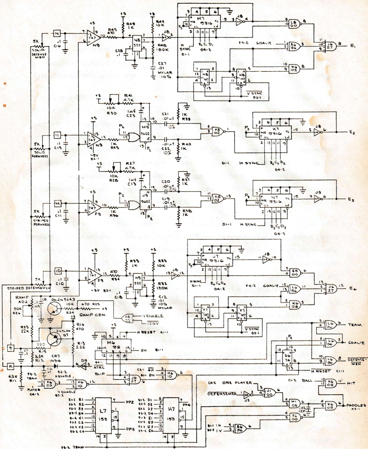
FIGURE 11. Players Circuit
