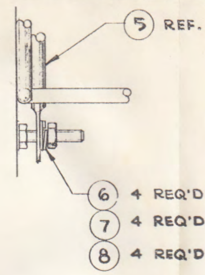
DETAIL "A"
