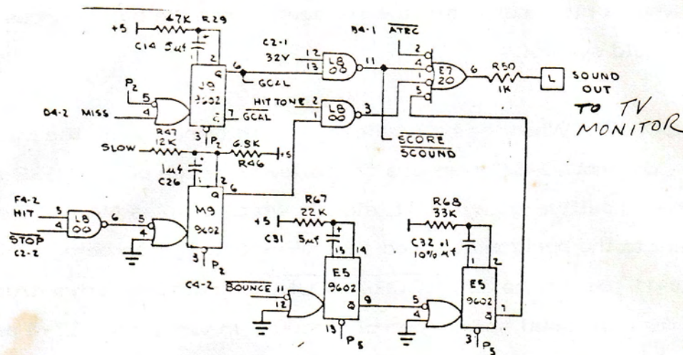
FIGURE 20. Sound Circuit
