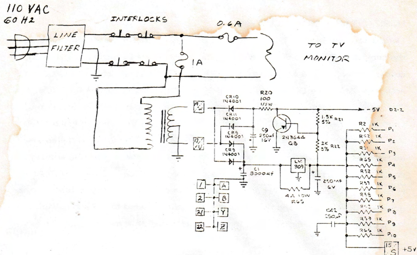
FIGURE 2. Power Supply
