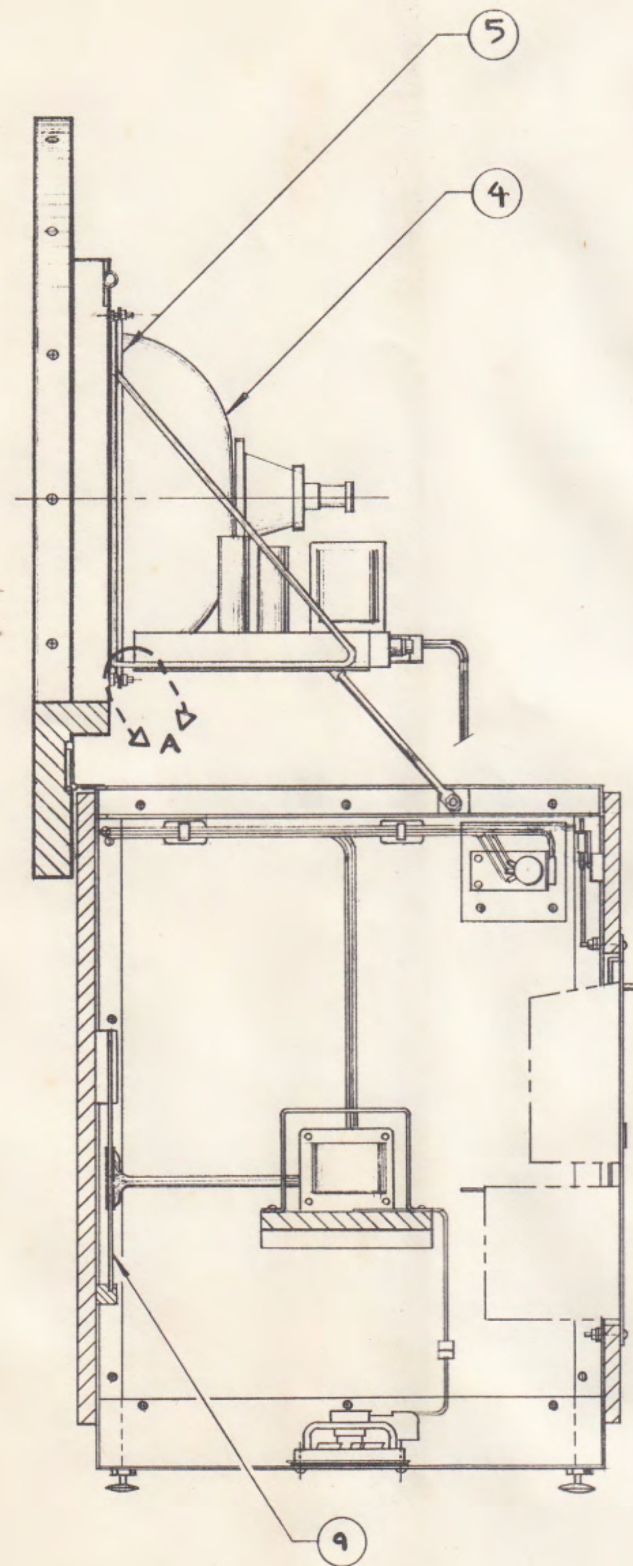
SECTION "B-B"
