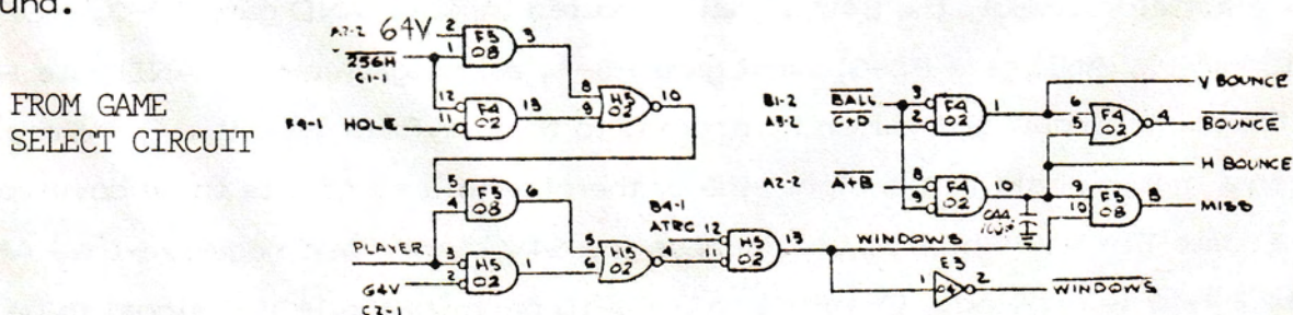
FIGURE 19. Window/Miss/Bounce Circuit
